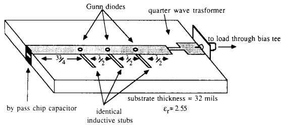
Fig. 3. Three Gunn diode power combining oscillator.
